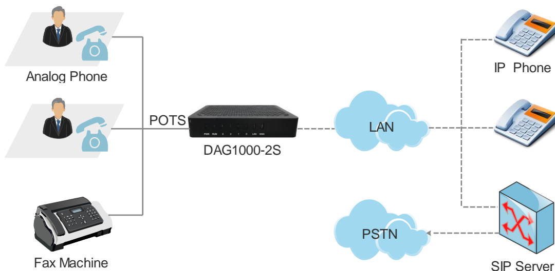
Figure 1-1 Application Scenario of DAG1000-1S/2S
